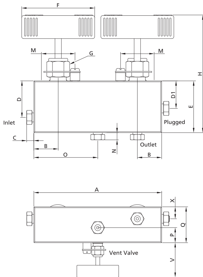
Bottom View
