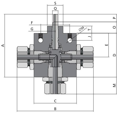
3-Way Valves
