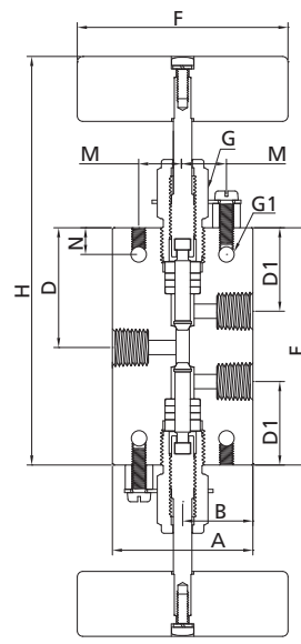
2 stem manifold
